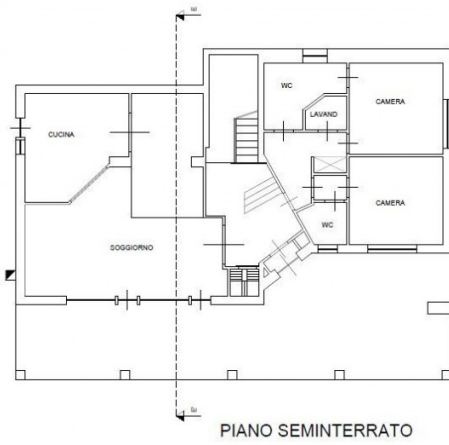
PIANO SEMINTERRATO
